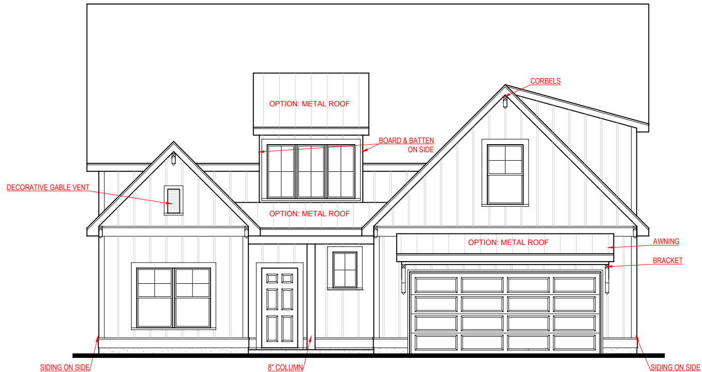
FRONT ELEVATION - A VERSION
