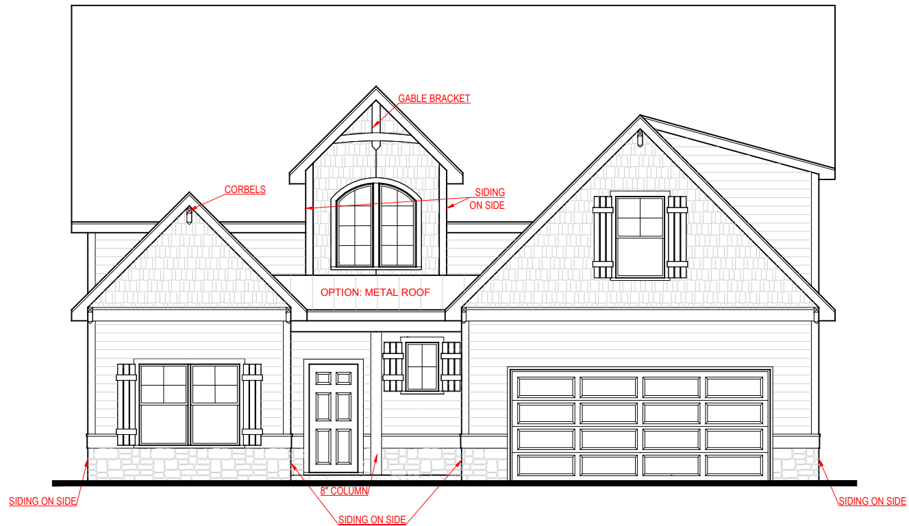
FRONT ELEVATION - B VERSION
