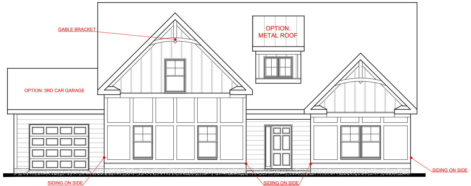
FRONT ELEVATION- A VERSION
