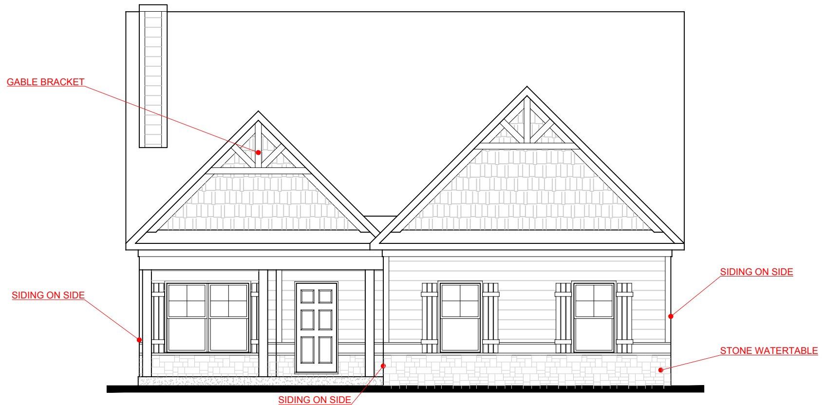
FRONT ELEVATION- B 3 CAR VERSION
