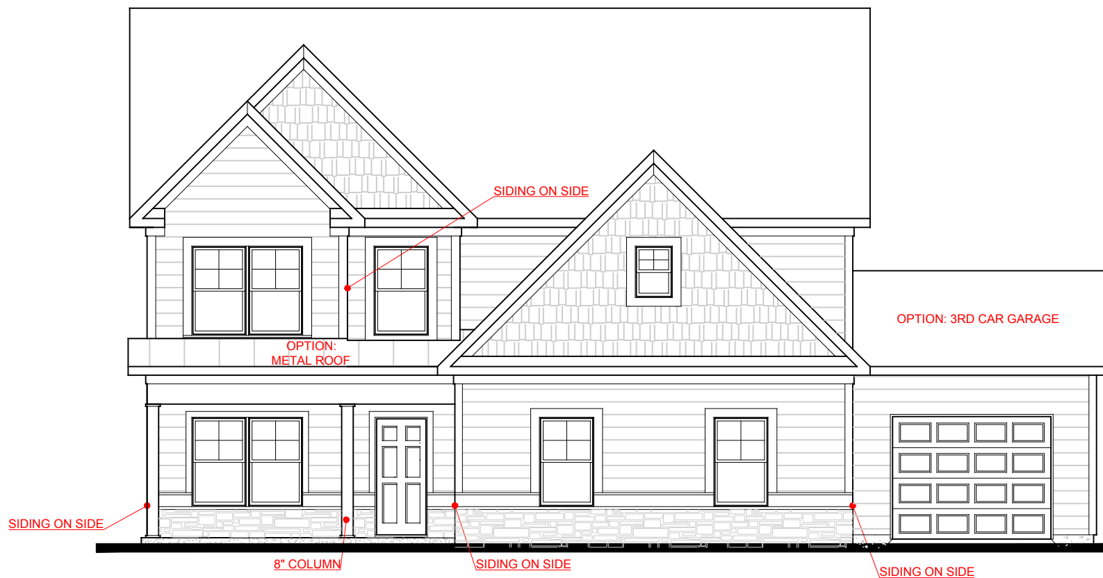
FRONT ELEVATION- B VERSION
