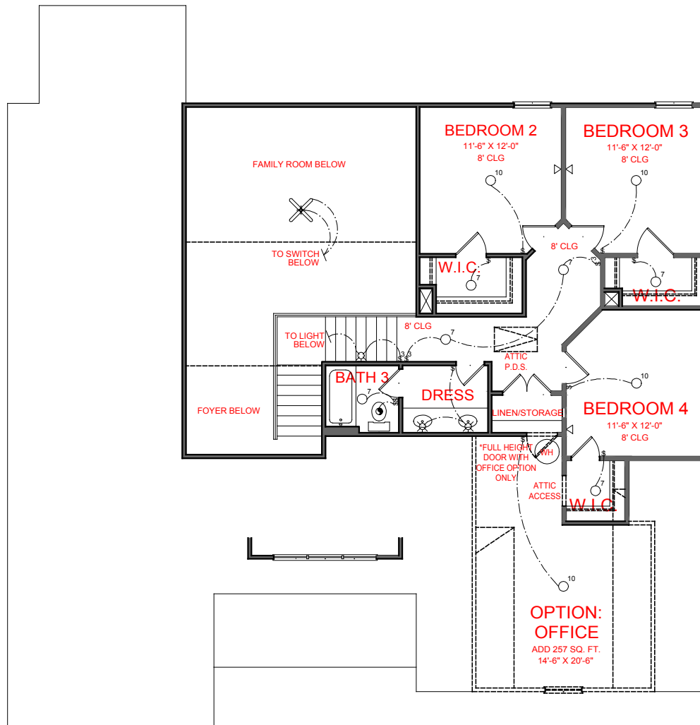
SECOND FLOOR PLAN- B & D VERSION
