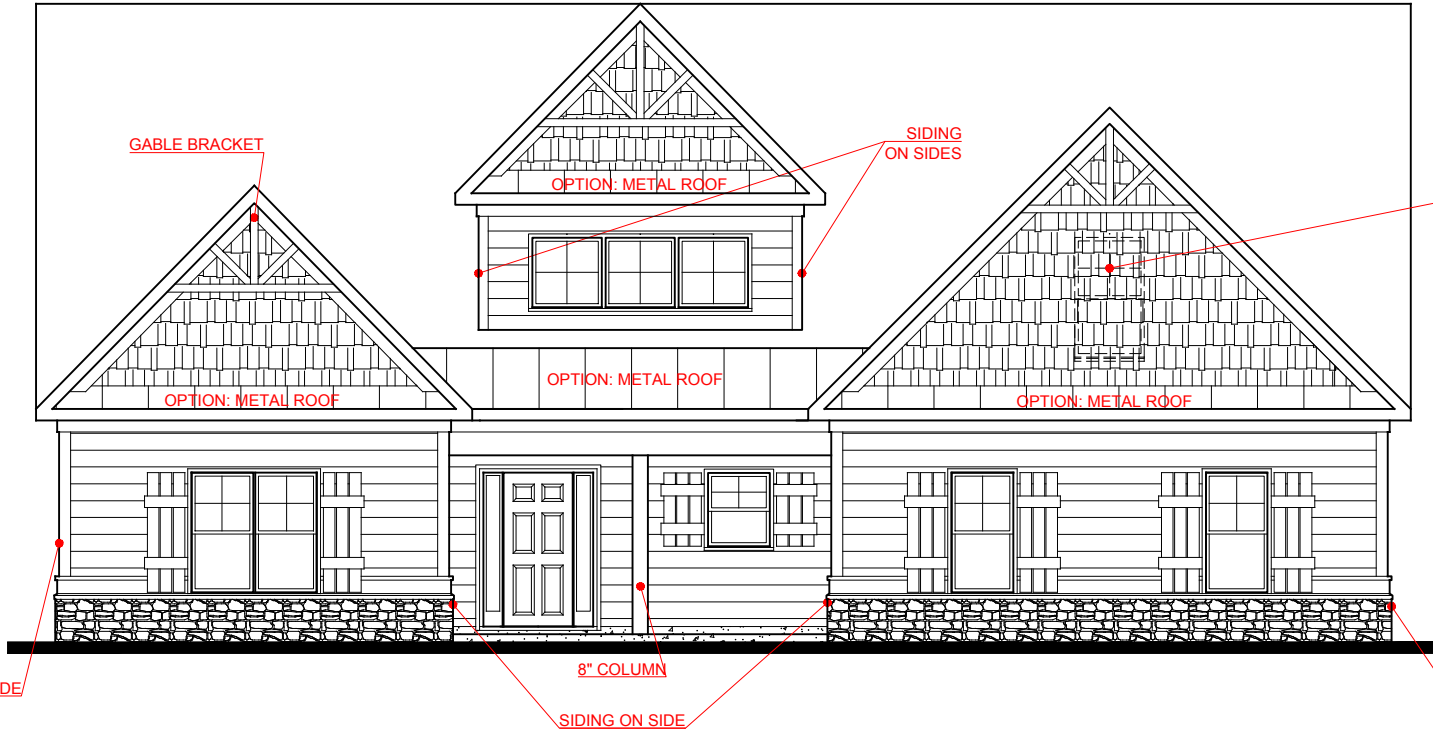
FRONT ELEVATION- B VERSION
