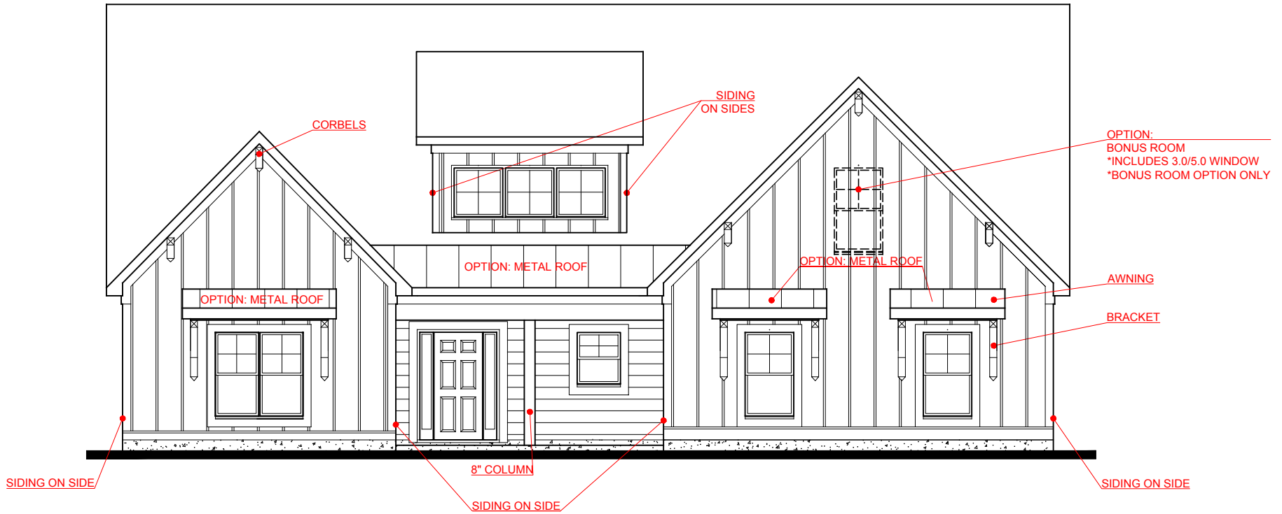
FRONT ELEVATION- A VERSION
