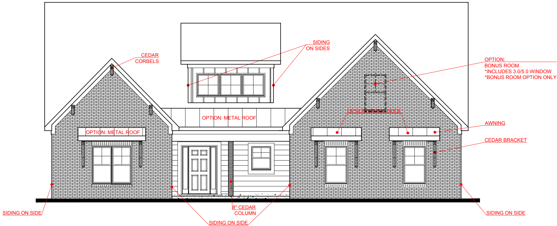
FRONT ELEVATION- F VERSION
