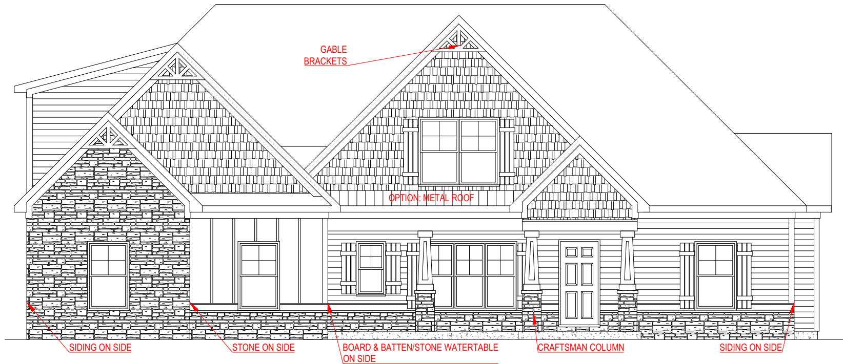
FRONT ELEVATION- C VERSION
