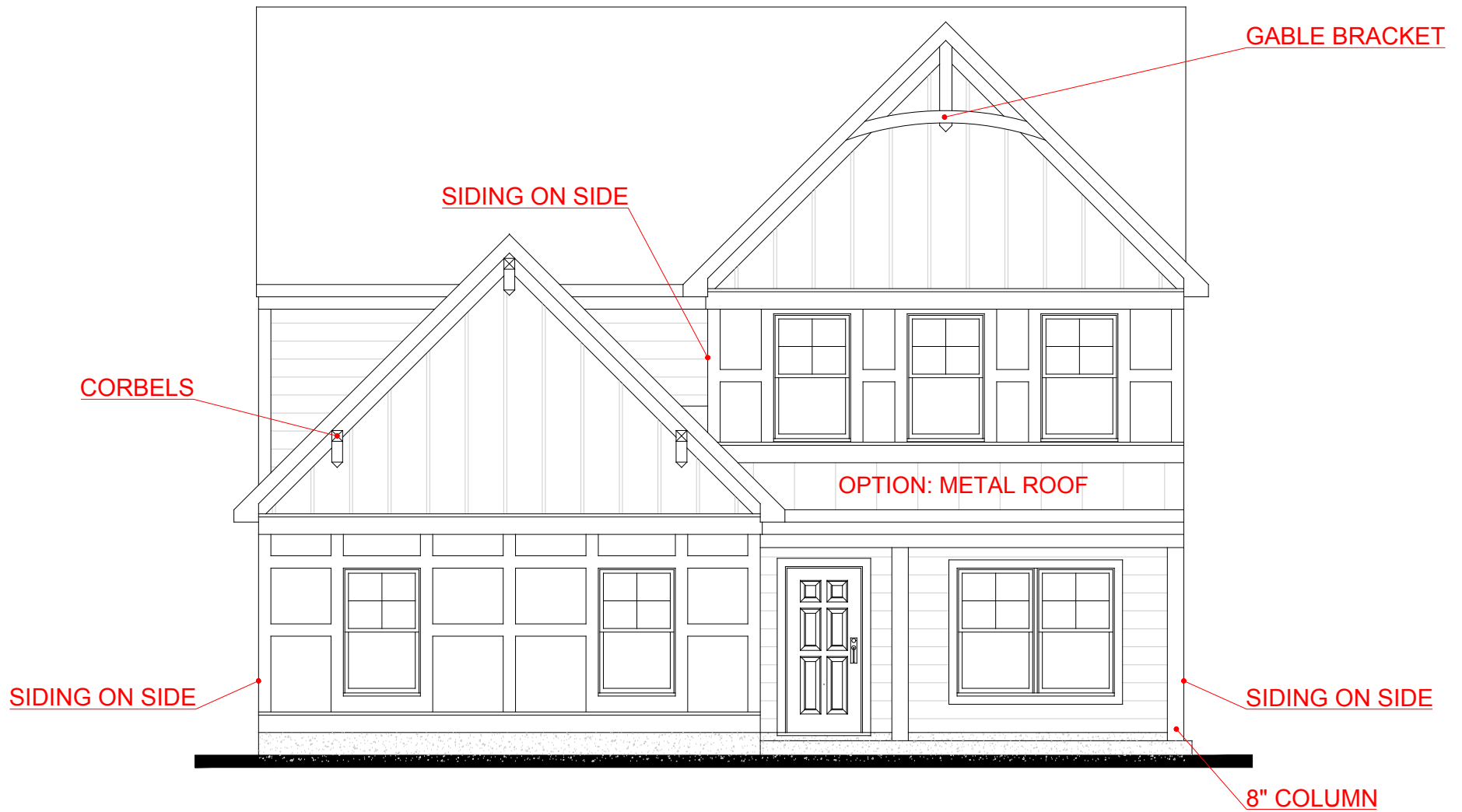
FRONT ELEVATION - A VERSION
