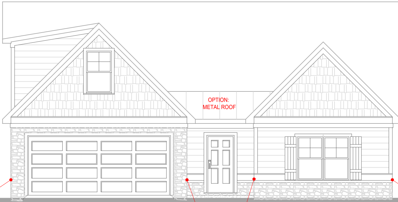
FRONT ELEVATION- B VERSION
