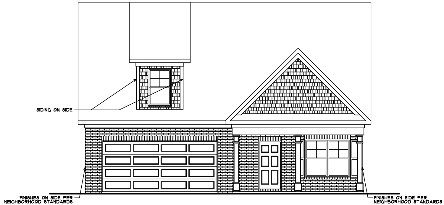
FRONT ELEVATION
