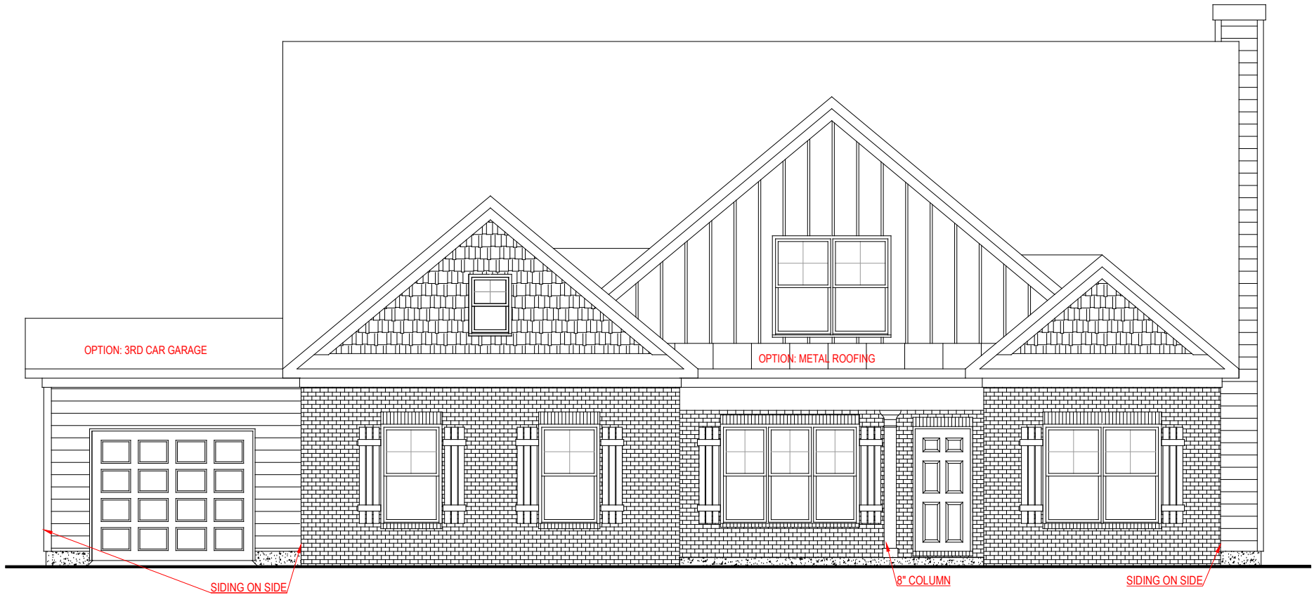
FRONT ELEVATION - B-D VERSION
