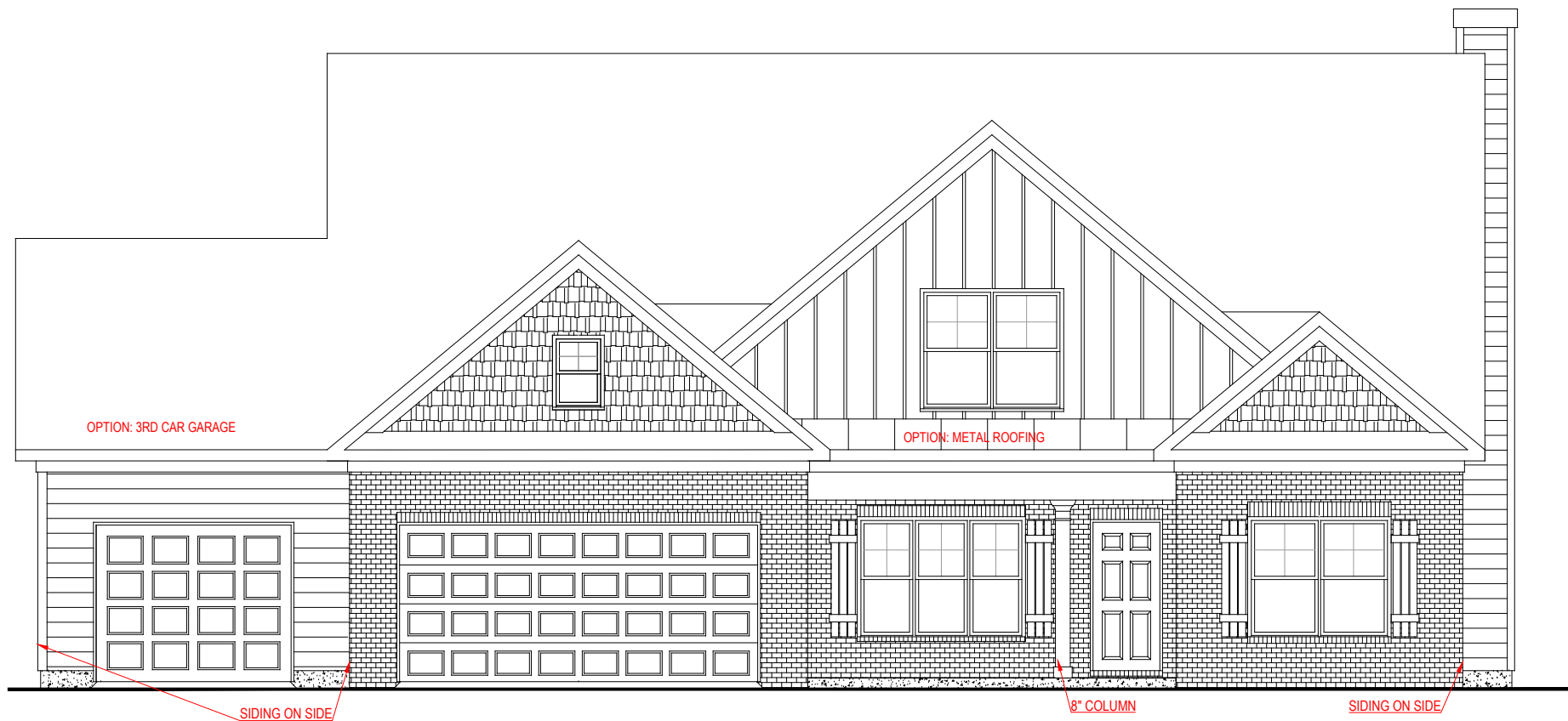
FRONT ELEVATION - B-D VERSION
