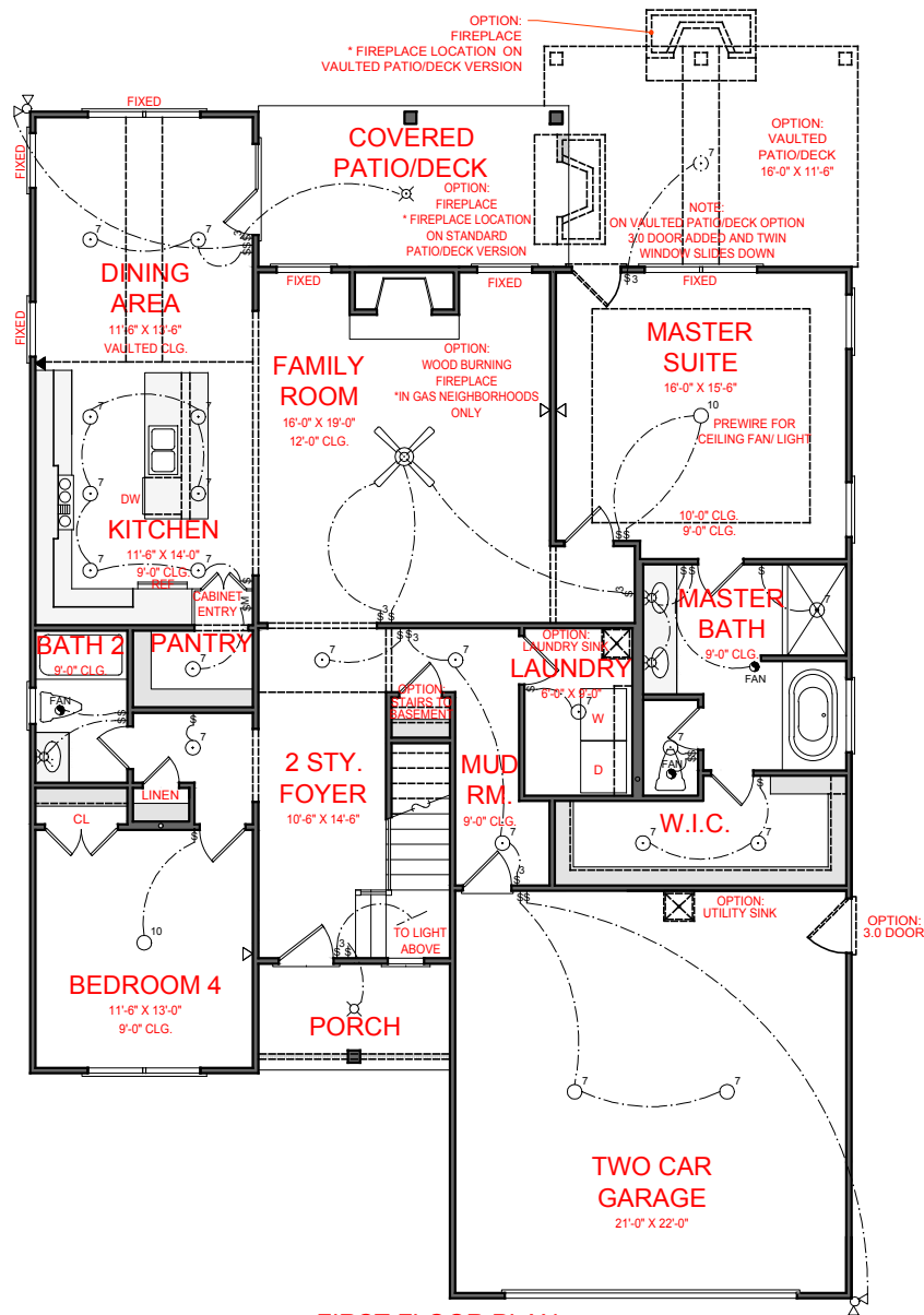
FIRST FLOOR PLAN * NO 1/2" FIRST FLOORS
