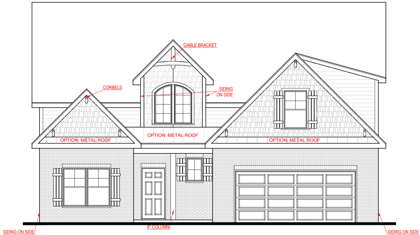
FRONT ELEVATION - D VERSION
