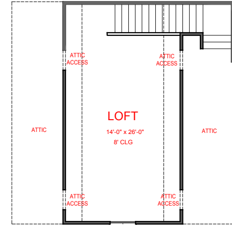
LOFT PLAN 364 SQ. FT.
