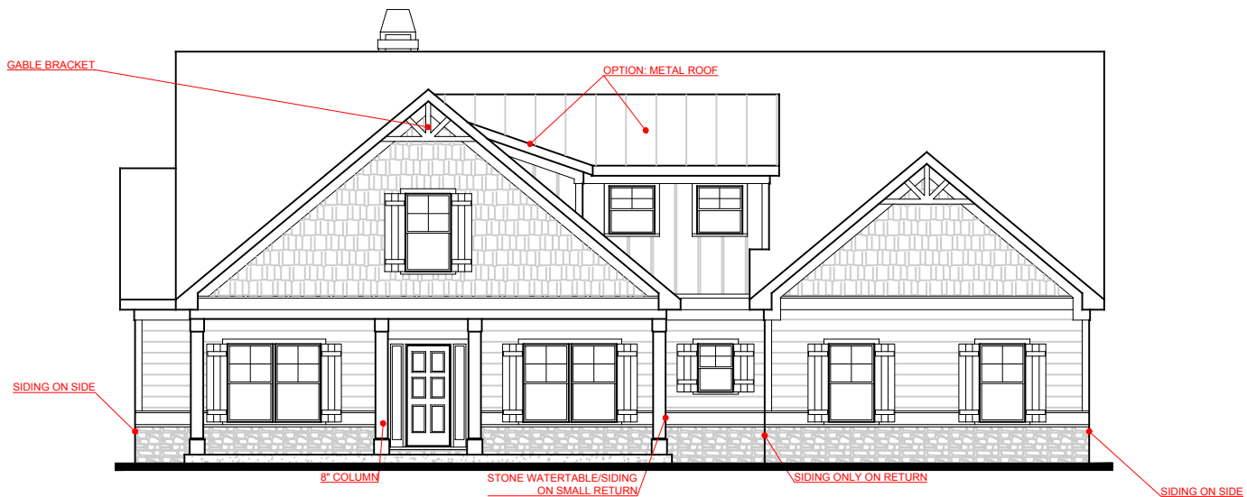
FRONT ELEVATION- B VERSION
