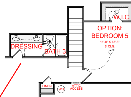
OPTION: BEDROOM 5 ADD 194 SQ. FT.
