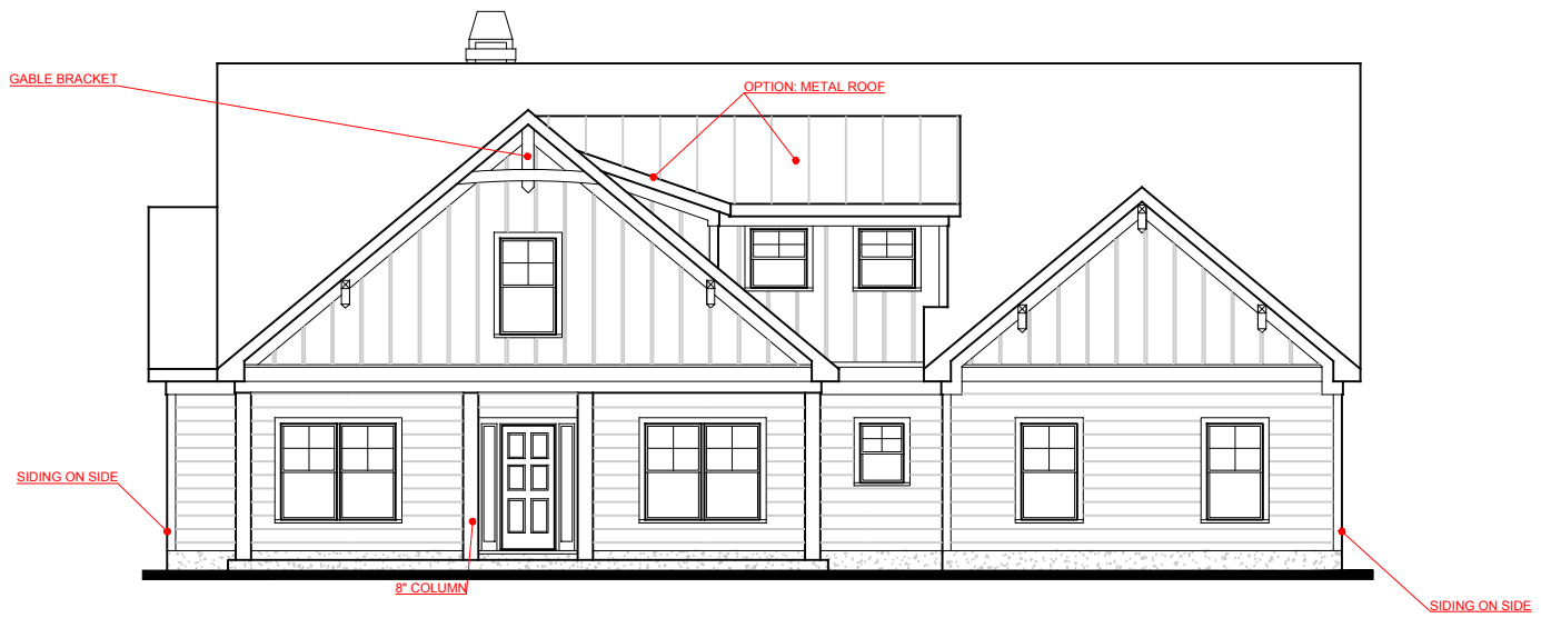
FRONT ELEVATION- A VERSION
