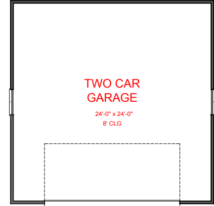
FLOOR PLAN 576 SQ. FT.
