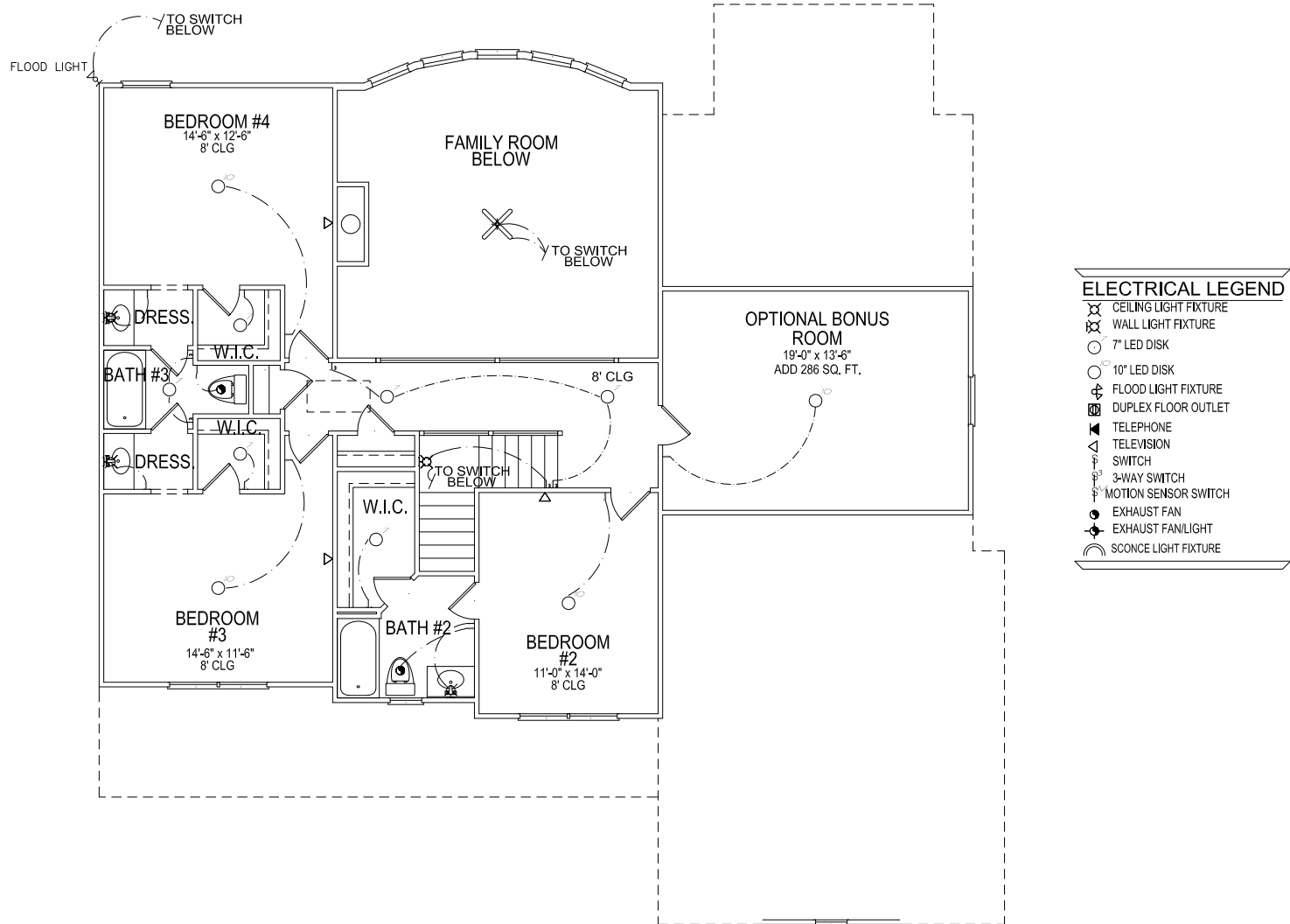
OPTIONAL SECOND FLOOR PLAN
